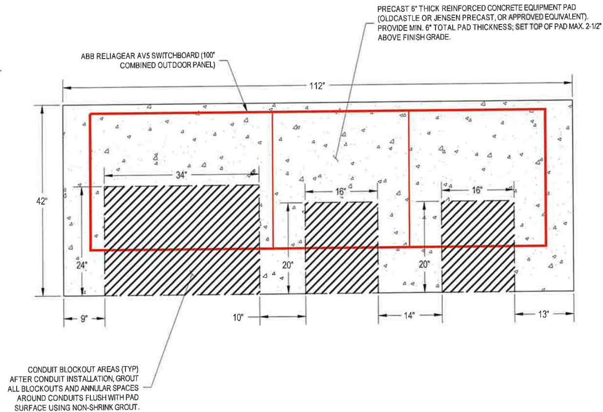
1 SWITCHBOARD PAD DETAIL SCALE: 1" = 10'
