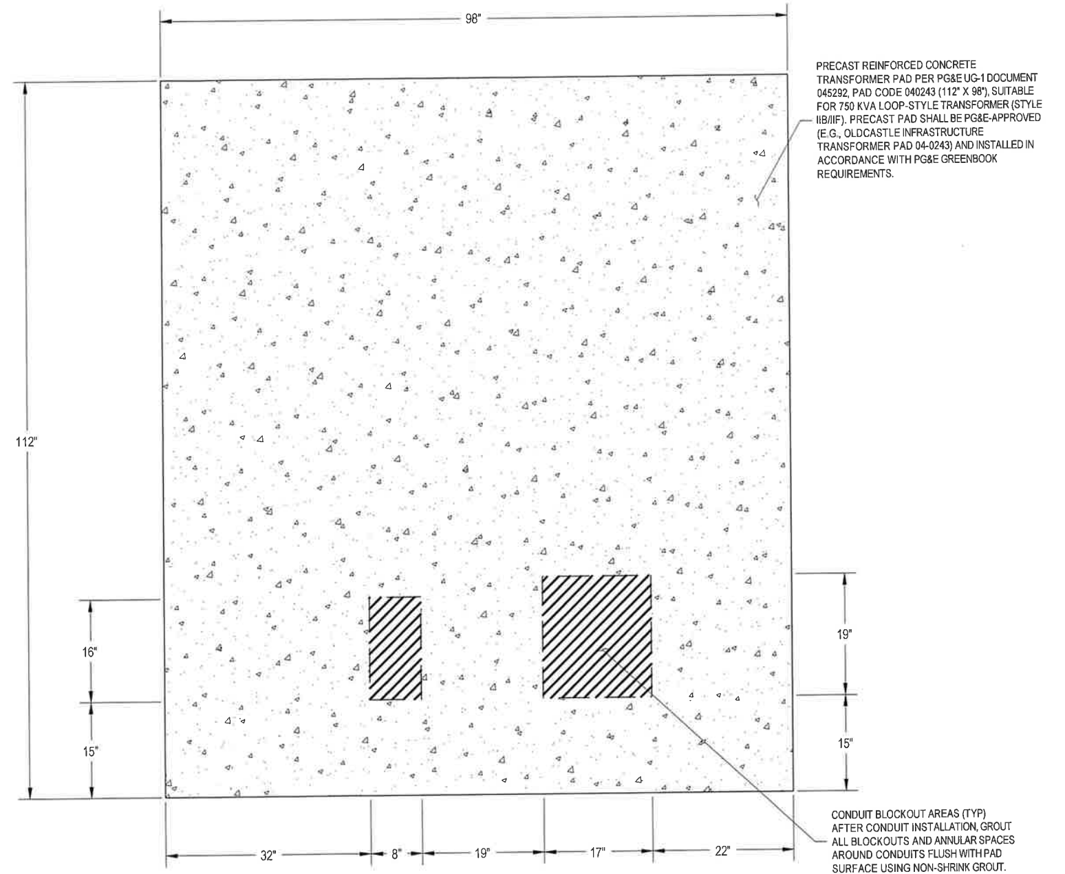
2 TRANSFORMER PAD DETAIL SCALE: 1" = 10'
